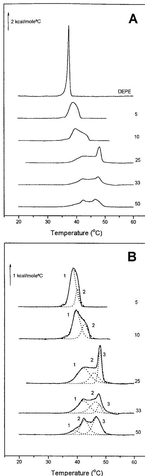
FIGURE 1 The gel-fluid transitions of pure DEPE and DEPE/ceramide mixtures as detected by differential scanning calorimetry. ( A ) Representative thermograms (second heating scan). ( B ) The same thermograms as in A , except the one corresponding to pure DEPE, drawn at a larger scale to show the component peaks (in broken lines). The component peaks are numbered 1, 2, 3, in increasing order of melting temperatures. The figures at the right of each thermogram represent the ceramide contents, in mole percentages.
