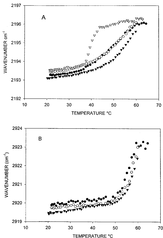
FIGURE 3 The gel-fluid transitions of pure d 54 -DPPC and d 54 -DPPC/ceramide mixtures as detected by IR spectroscopy. The maximal frequencies of the asymmetric C—H or C—D stretching bands are plotted as a function of temperature (data from the second heating scan). ( A ) C—D vibrations of d 54 -DPPC. ▽, pure phospholipid; ●, ○, ▼, phospholipid/ceramide mixtures containing, respectively, 15, 20, and 25 mol % ceramide. ( B ) C—H vibrations of ceramide chains. Symbols are as in A .
