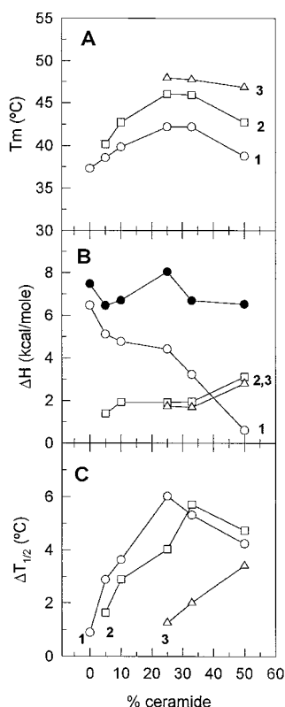
FIGURE 2 Thermodynamic parameters of the gel-fluid transitions of pure DEPE and DEPE/ceramide mixtures. Data are derived from thermograms as shown in Fig. 1. ( A ) Midpoint transition temperatures of the component peaks. ○, peak 1; □, peak 2; △, peak 3. ( B ) Transition enthalpies of the overall transition and of its components. ●, overall transition \Delta H ; other symbols as in A . ( C ) Width at mid-height of the component transition peaks. Symbols are as in A .
